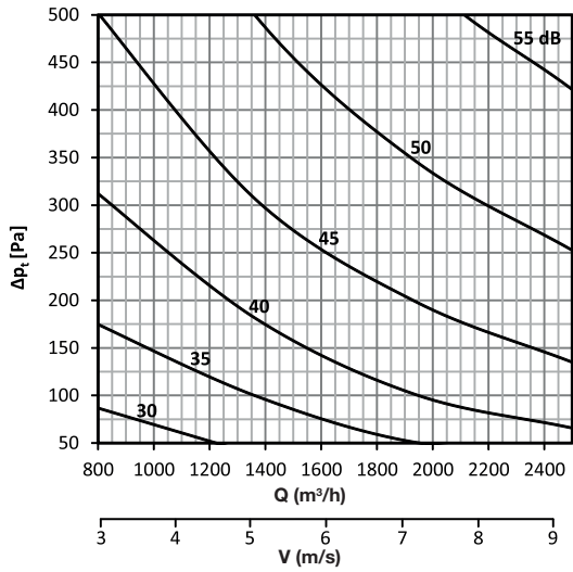
DAC-R 300 x 250
