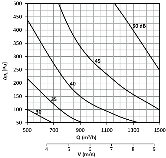
DAC-R 300 x 150
