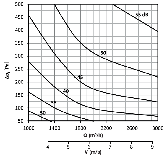
DAC-R 300 x 300
