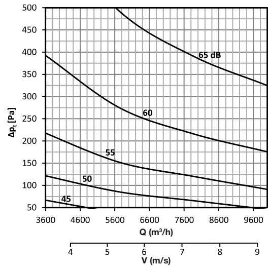
DAC-R 600 x 500
