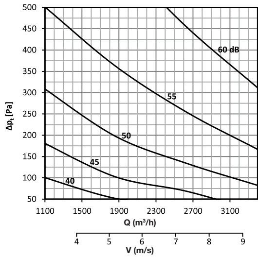
DAC-R 500 x 200
