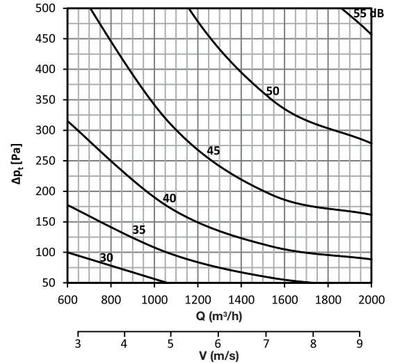
DAC-R 300 x 200
