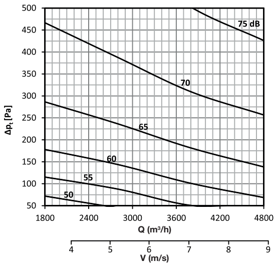
DAC-R 500 x 300
