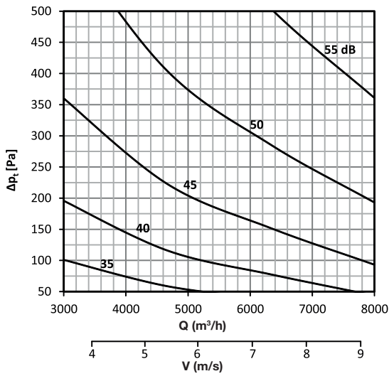
DAC-R 600 x 400
