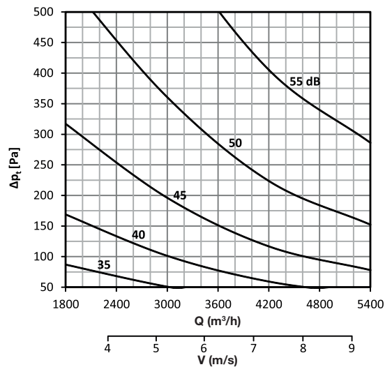
DAC-R 400 x 400
