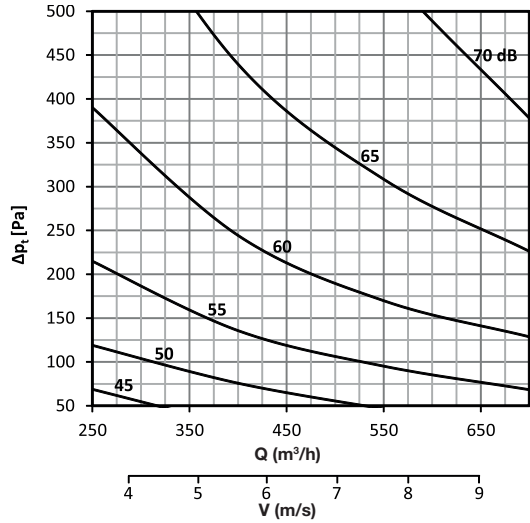
DAC-R 200 x 100
