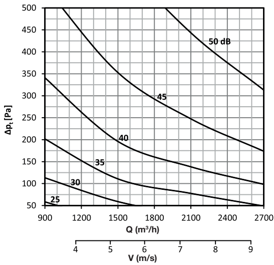
DAC-R 400 x 200
