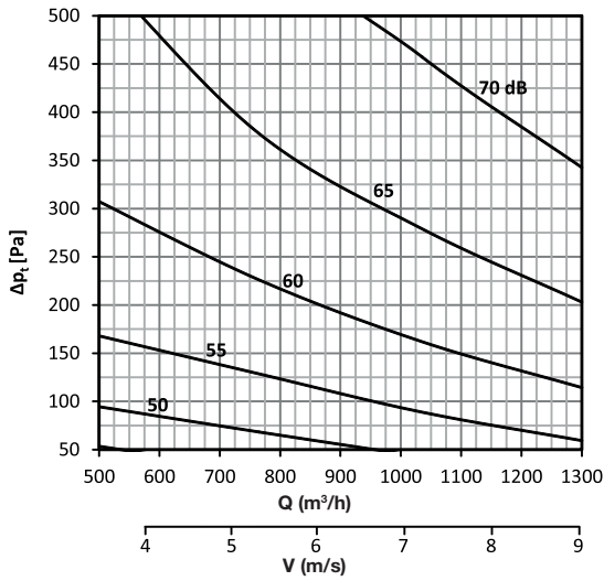
DAC-R 200 x 200
