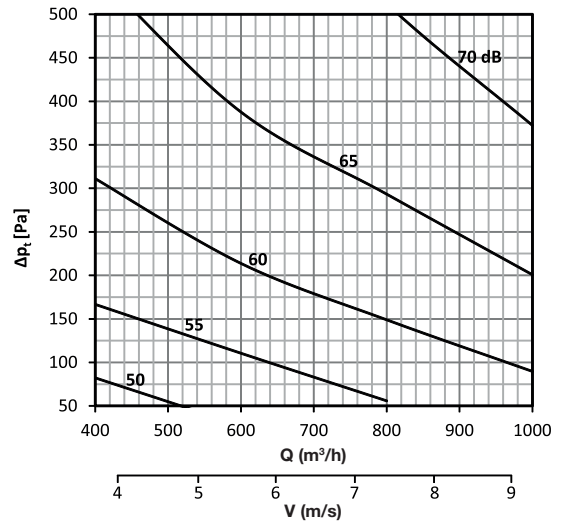
DAC-R 300 x 100
