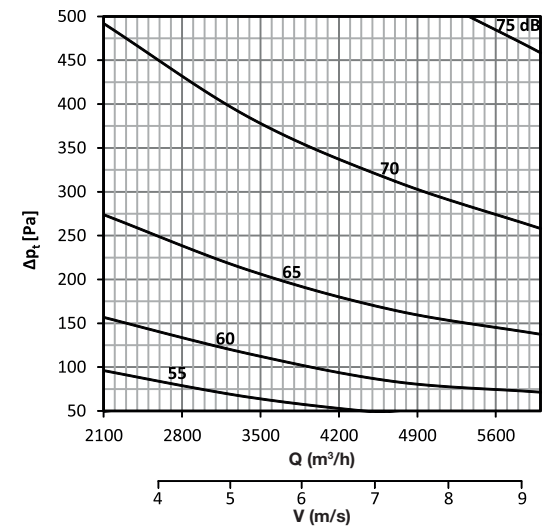
DAC-R 600 x 300
